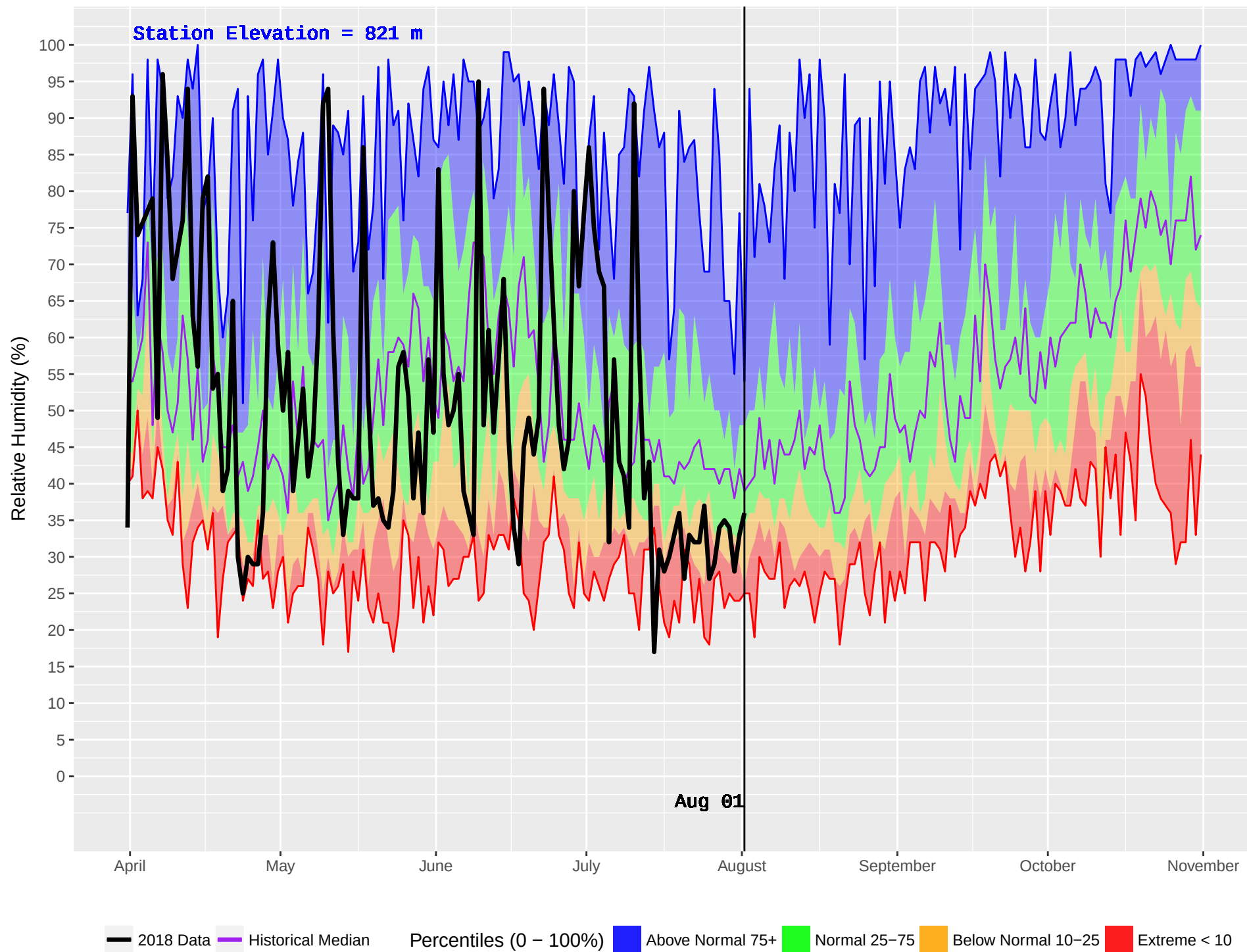
AKOKLI CREEK (838) : Historical (2003–2016) and Current (2018) Daily Relative Humidity
